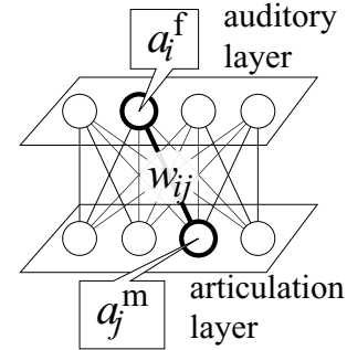
Figure 3: Connections between the auditory layer and the articulation one.
